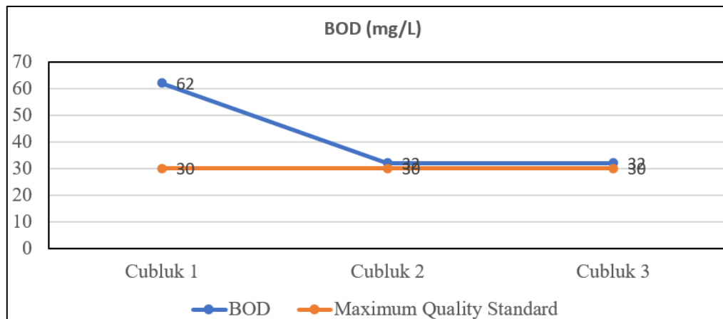
Figure 5. Laboratory Test Results on BOD Parameter Samples
