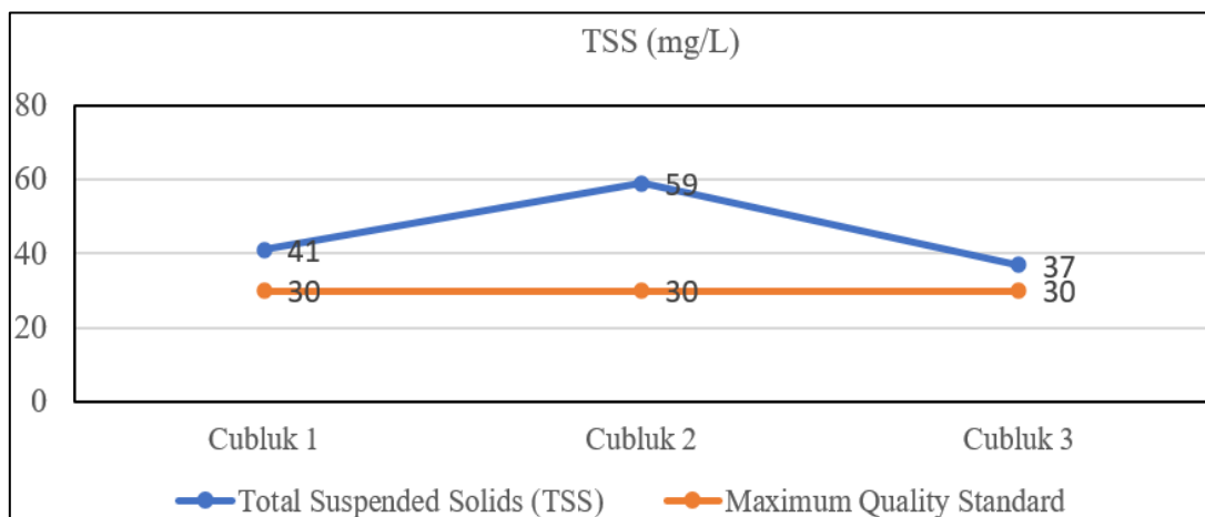
Figure 3. Laboratory Test Results on TSS Parameter Samples
